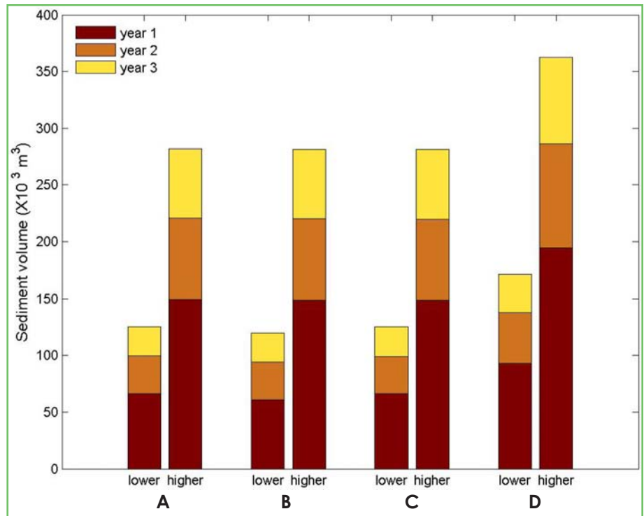
Predicted sediment volume for the Port and marina region by year and in cubic meters for Alternatives A to D. [Report Figure 4.8]
