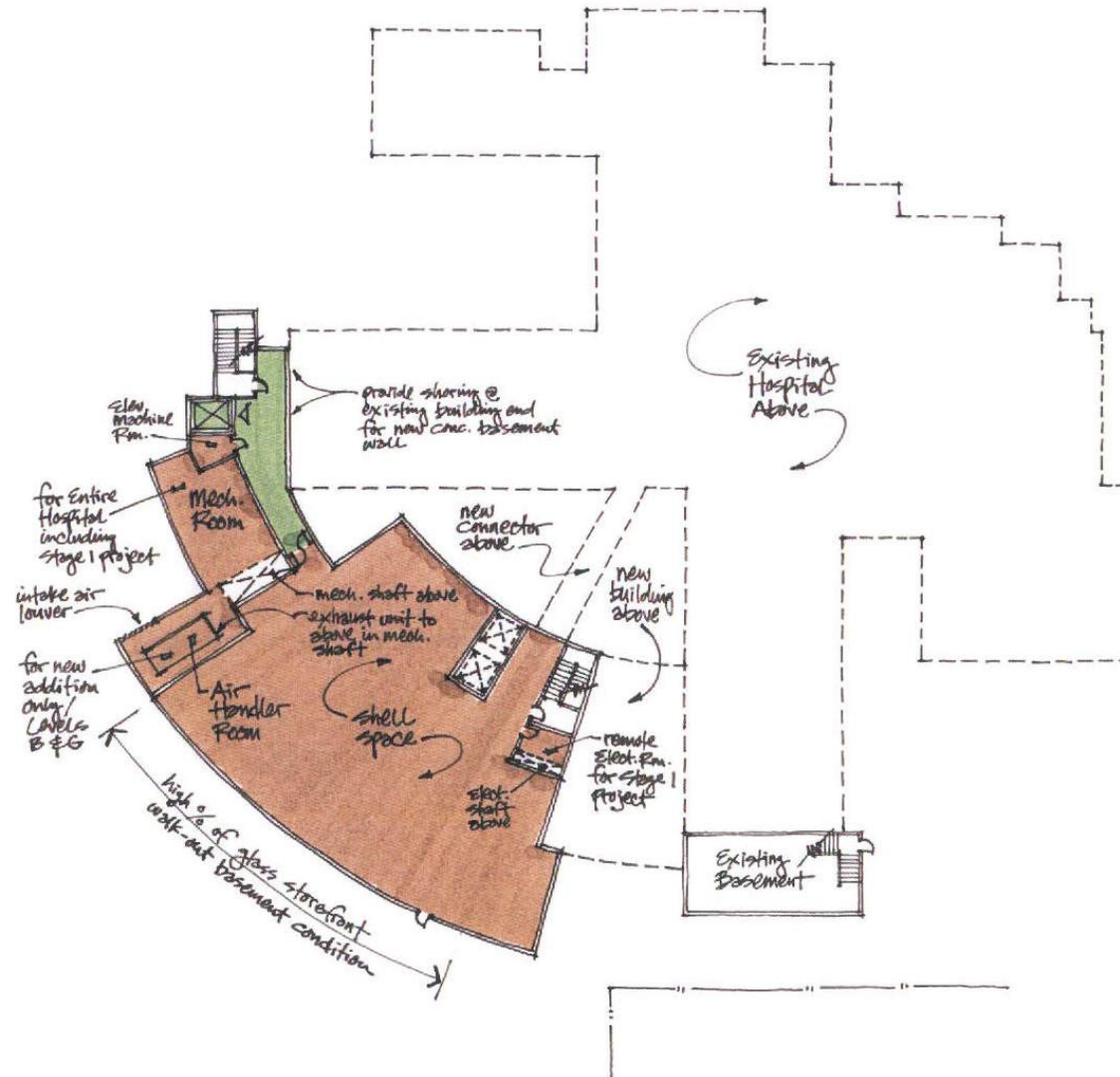
CONCEPTUAL BASEMENT FLOOR PLAN
