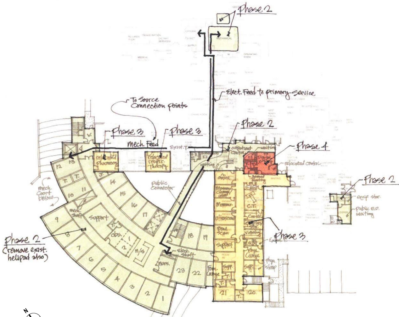
CONCEPTUAL GROUND FLOOR PHASING PLAN
